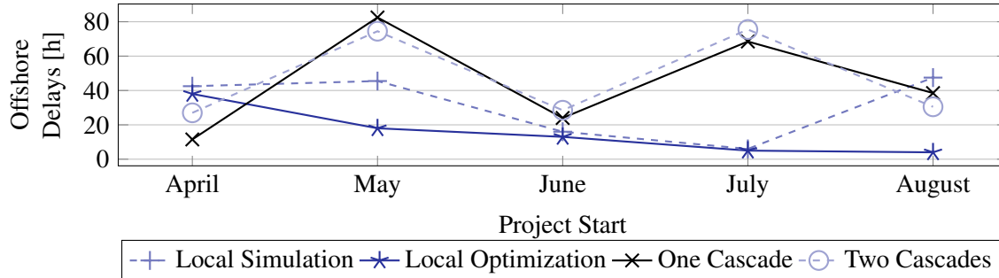
Figure 5: Installation duration for 50 OWTs by method and starting month.
